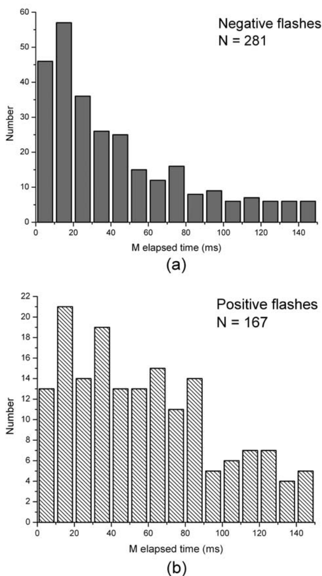
Figure 1. M component elapsed time since the RS for (a) negative (81% of the data set by Campos et al. [2007]) and (b) positive flashes (88% of the data set by Campos et al. [2009]). Adapted from Campos et al. [2009, Figure 3 insets] with permission from Elsevier.
