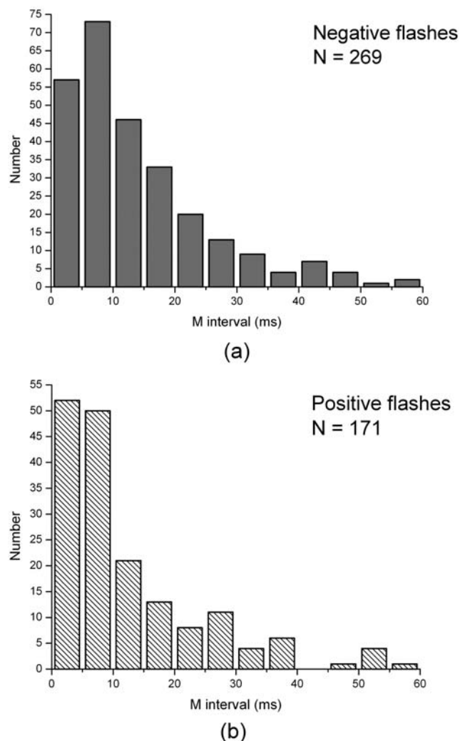
Figure 2. Time interval between successive M components for (a) negative (93% of the data set by Campos et al. [2007]) and (b) positive flashes (99% of the data set by Campos et al. [2009]). Adapted from Campos et al. [2009, Figure 5 insets] with permission from Elsevier.
